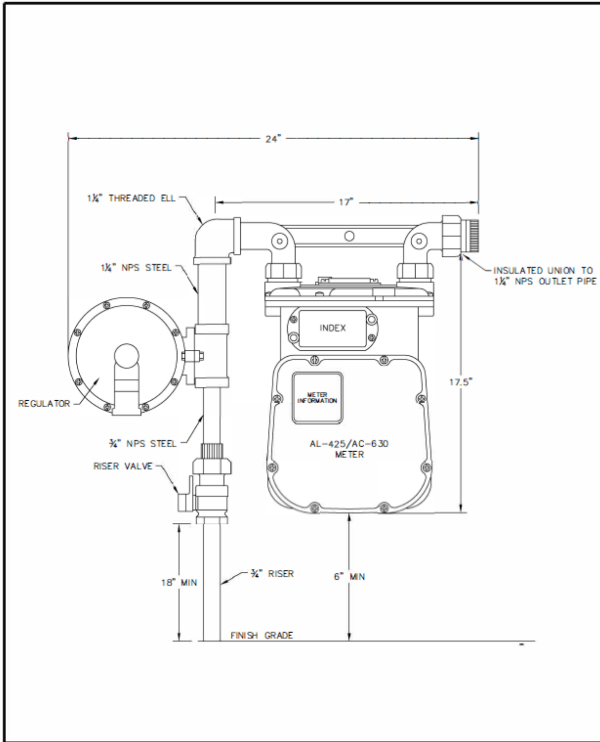
Figure A-5 AC-425/ AC630 Single Meter Manifold Detail
