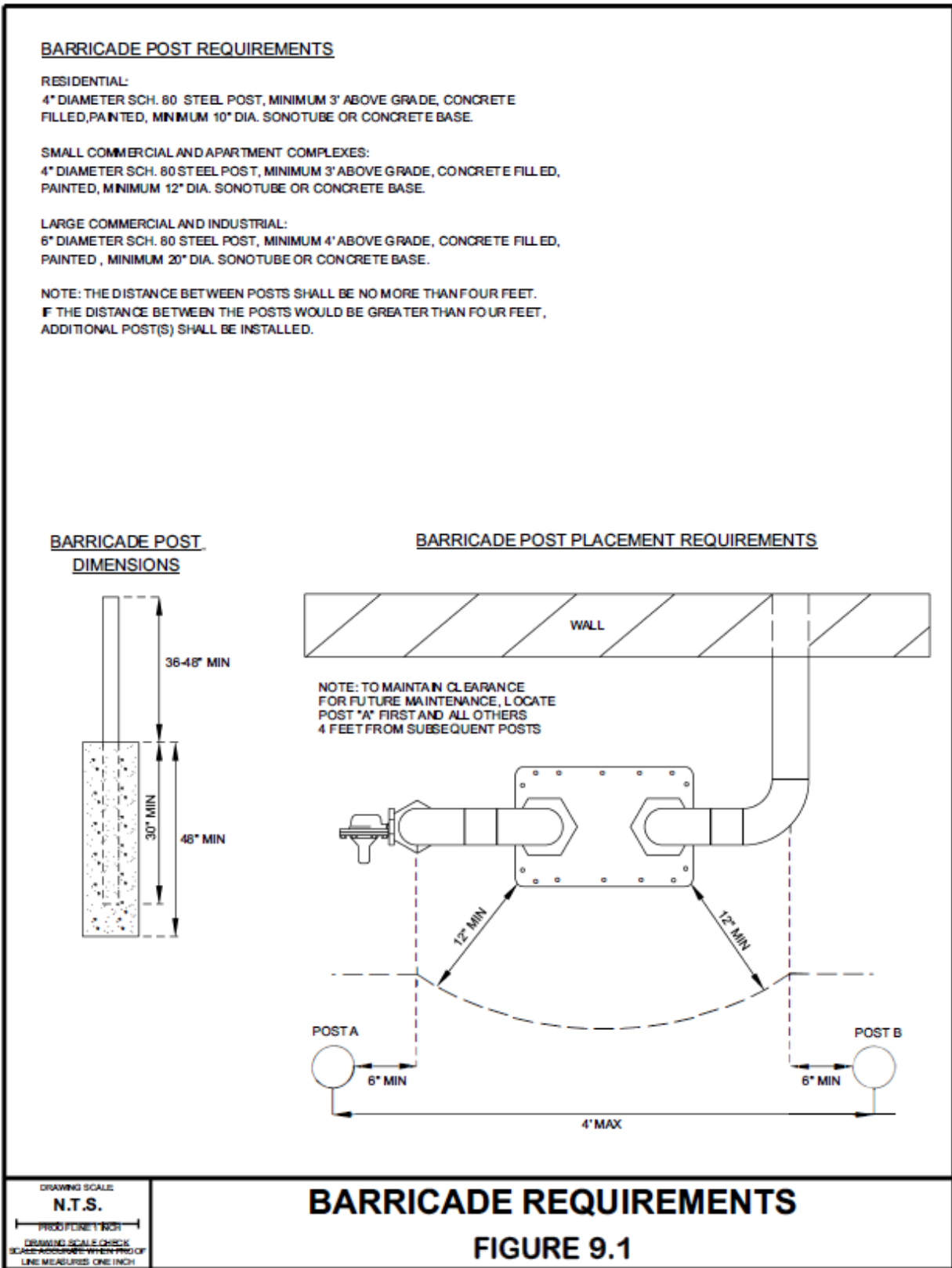
Figure 9.1 Barricade Requirements
