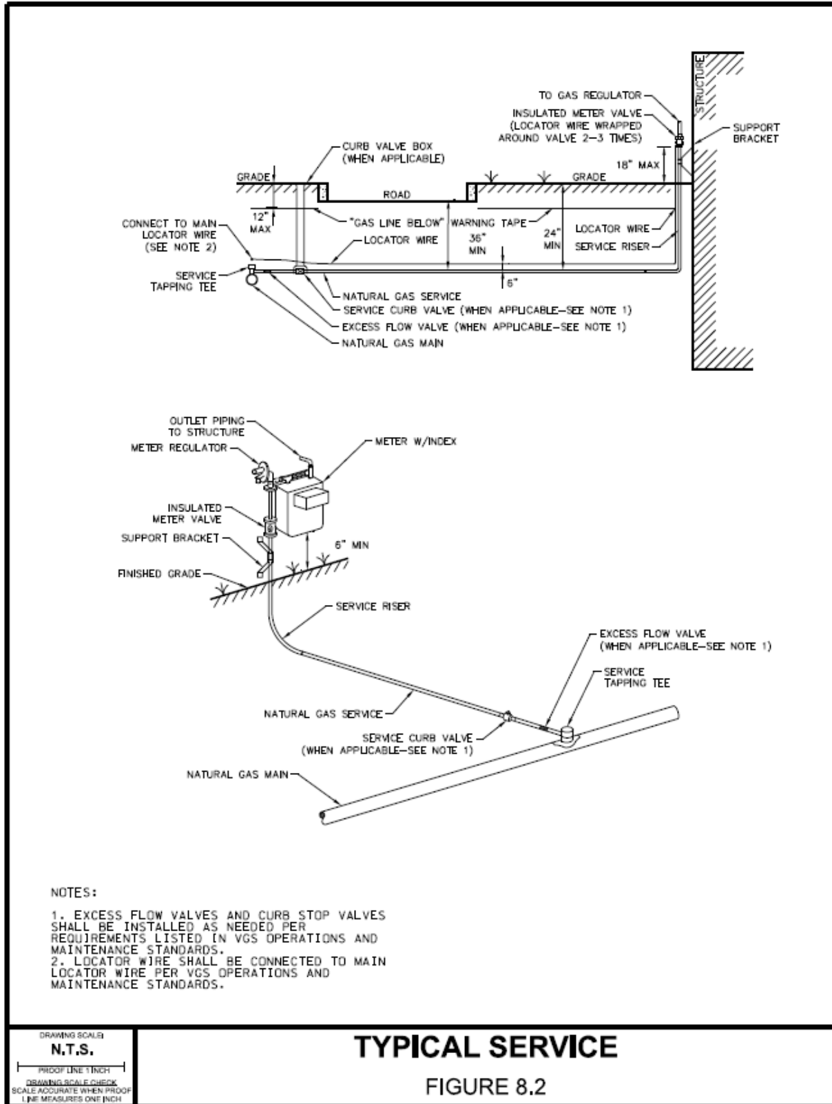
Figure 8-2 Typical Service
