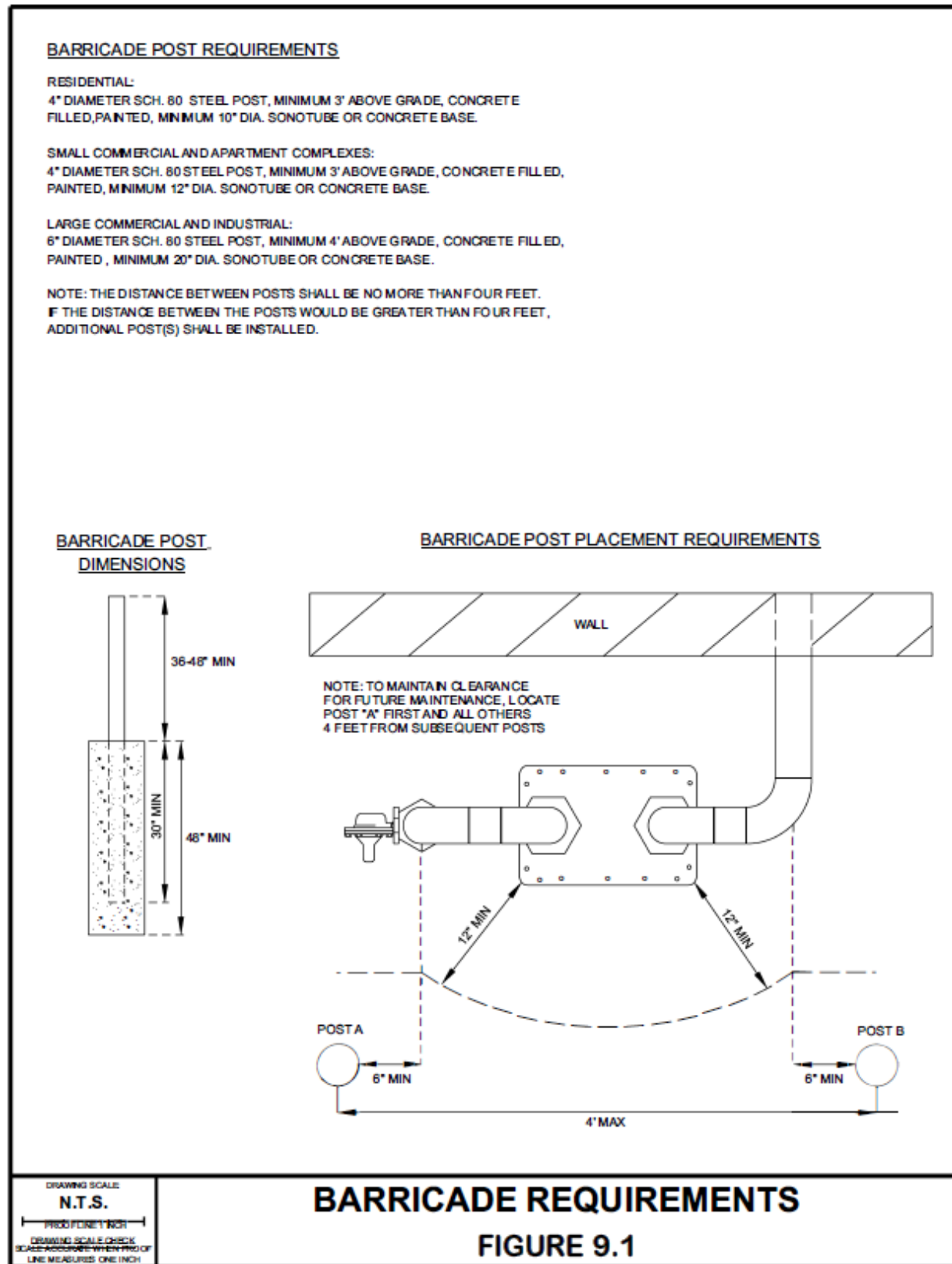
Figure 9.1 Barricade Requirements
