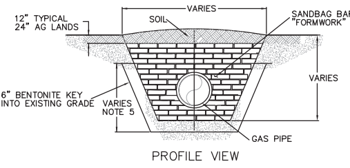
PROFILE VIEW
