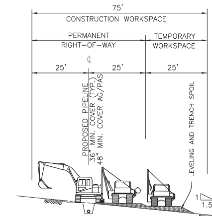
CONSTRUCTION TYPE 6C NOT TO SCALE
