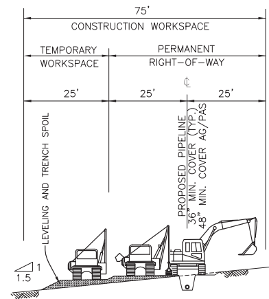
CONSTRUCTION TYPE 6A NOT TO SCALE
