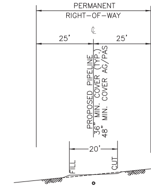
CONSTRUCTION TYPE 6B NOT TO SCALE
